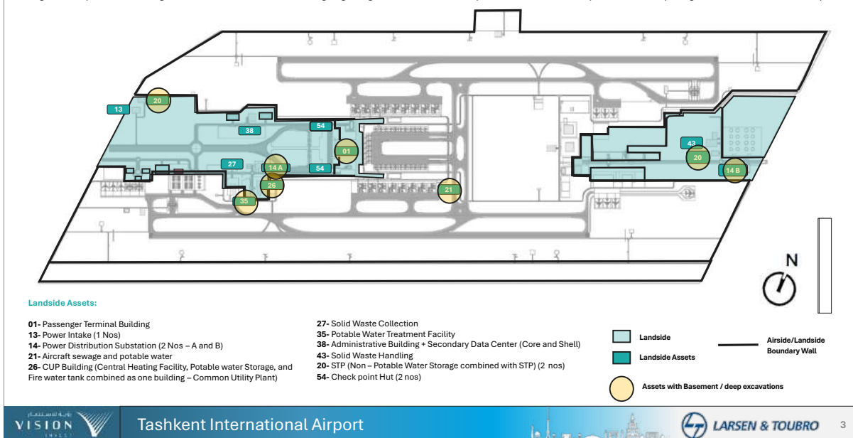
Figure 12: Airport Terminal main Facilities with sub-water table excavations
