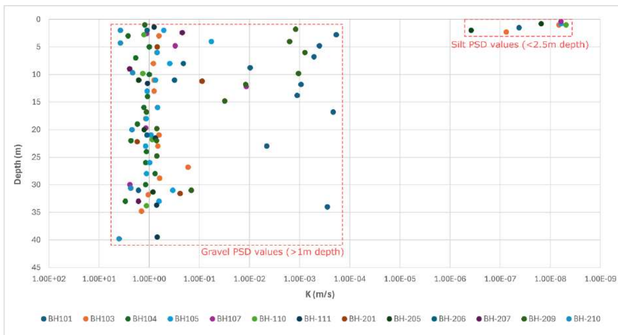
Figure 7: Kozeny-Carman analysis
