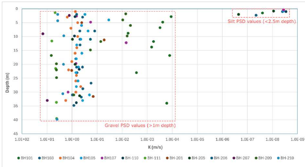
Figure 6: Hazen analysis
