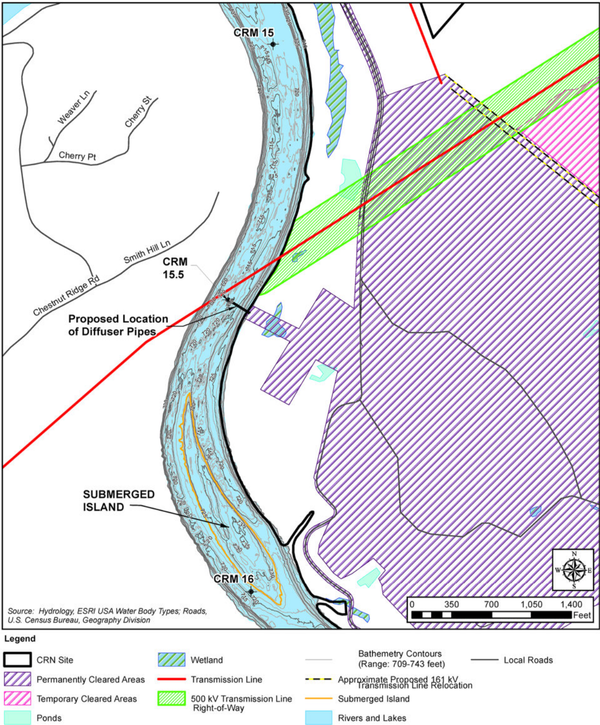
Figure 2-18 Bathymetry of the Clinch River at the CRN Site Discharge Location (contours are elevation in feet) (Source: TVA 2019-TN5854)
