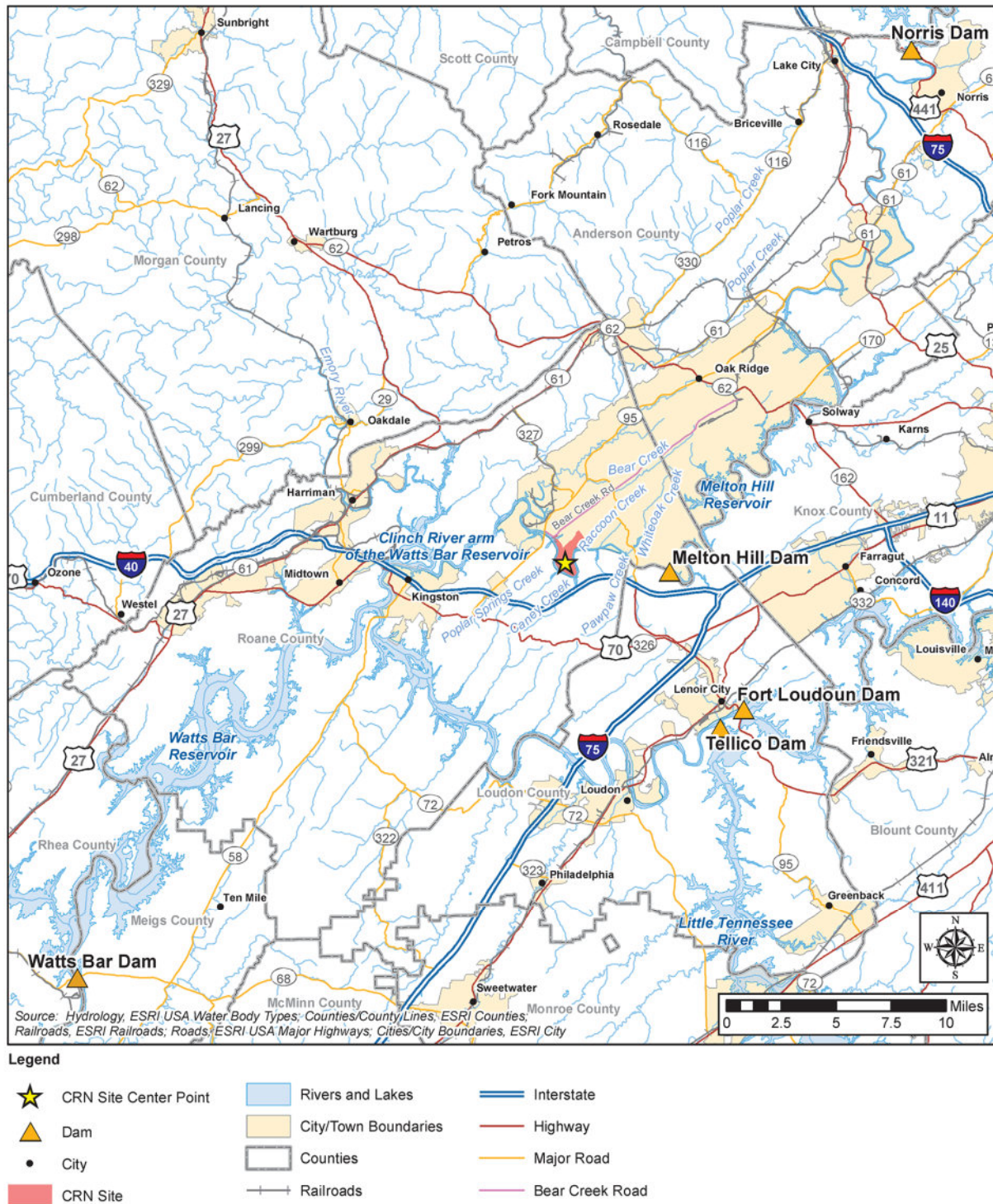
Figure 2-13 Locations of Dams that Influence Flows at the CRN Site (Source: TVA 2019-TN5854)
