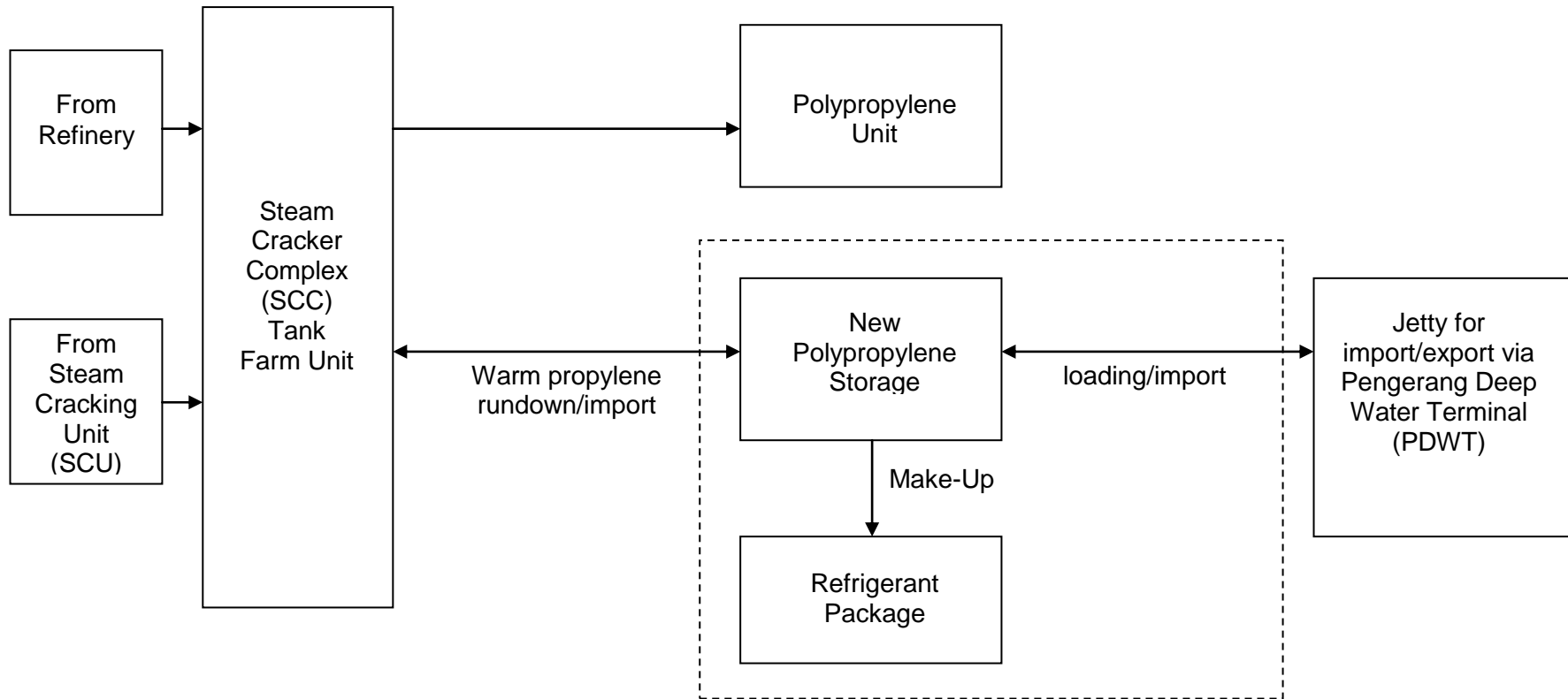
Figure 2-18: Process Flow Diagram for New Polypropylene Storage
