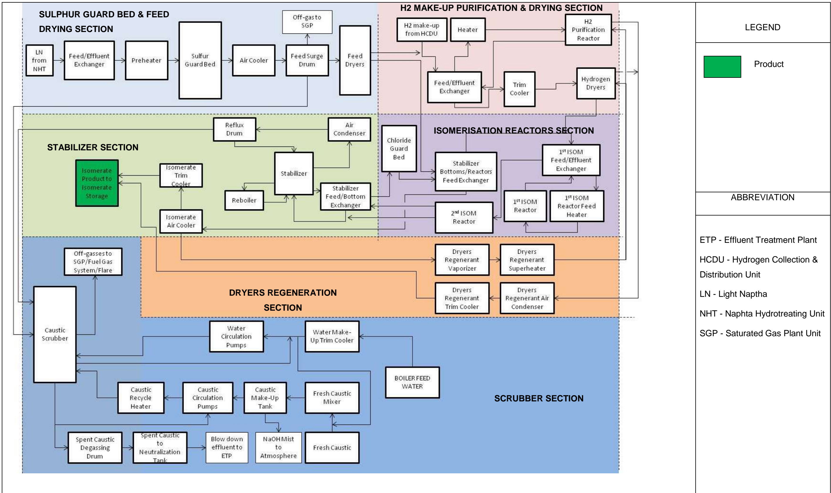
Figure 2-12: Overall Block Flow Diagram for Isomerisation Unit
