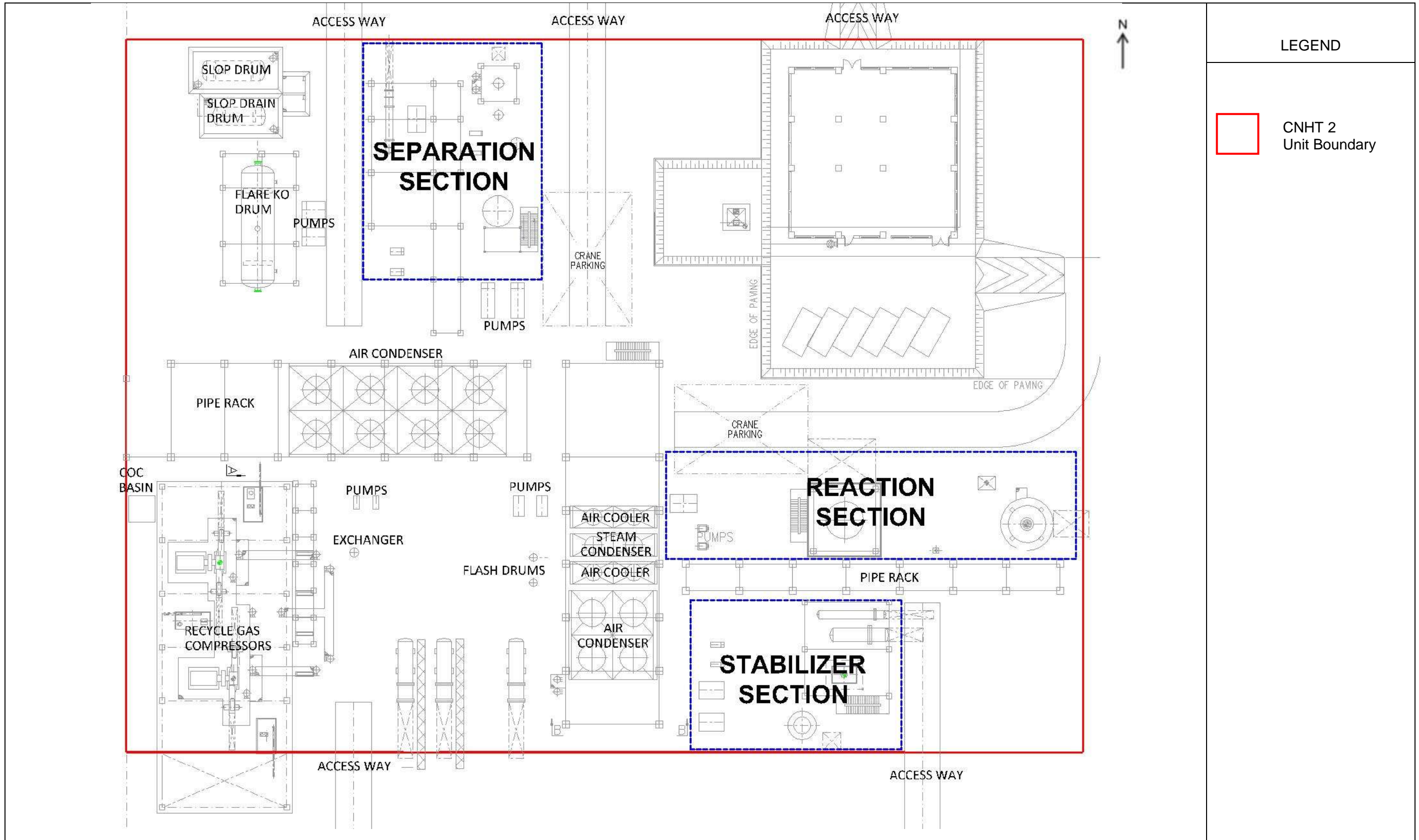
Figure 2-7: Layout Plan of Unit CNHT 2
