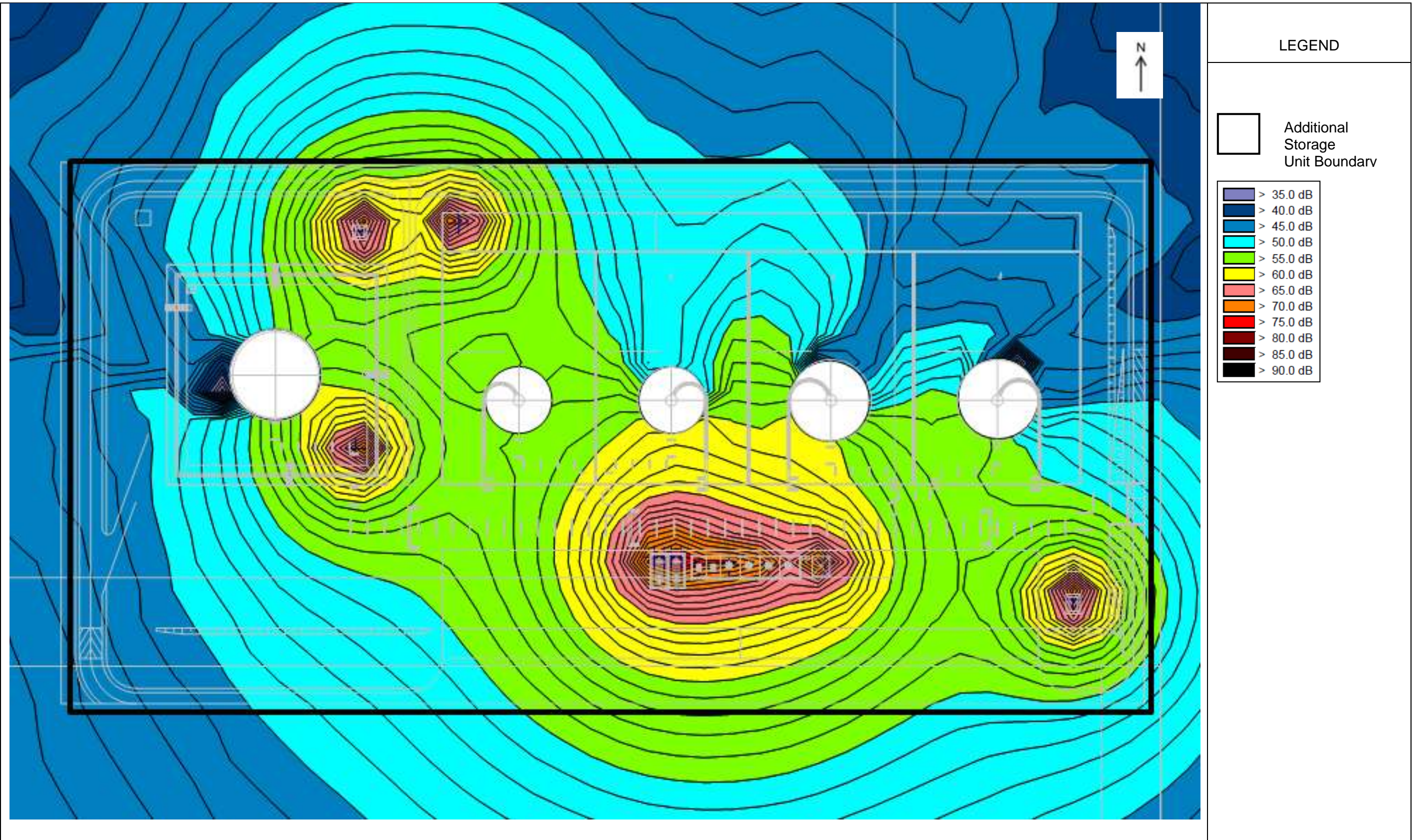
Figure 4-5: Noise Contour Generated from the Additional Storage Unit
