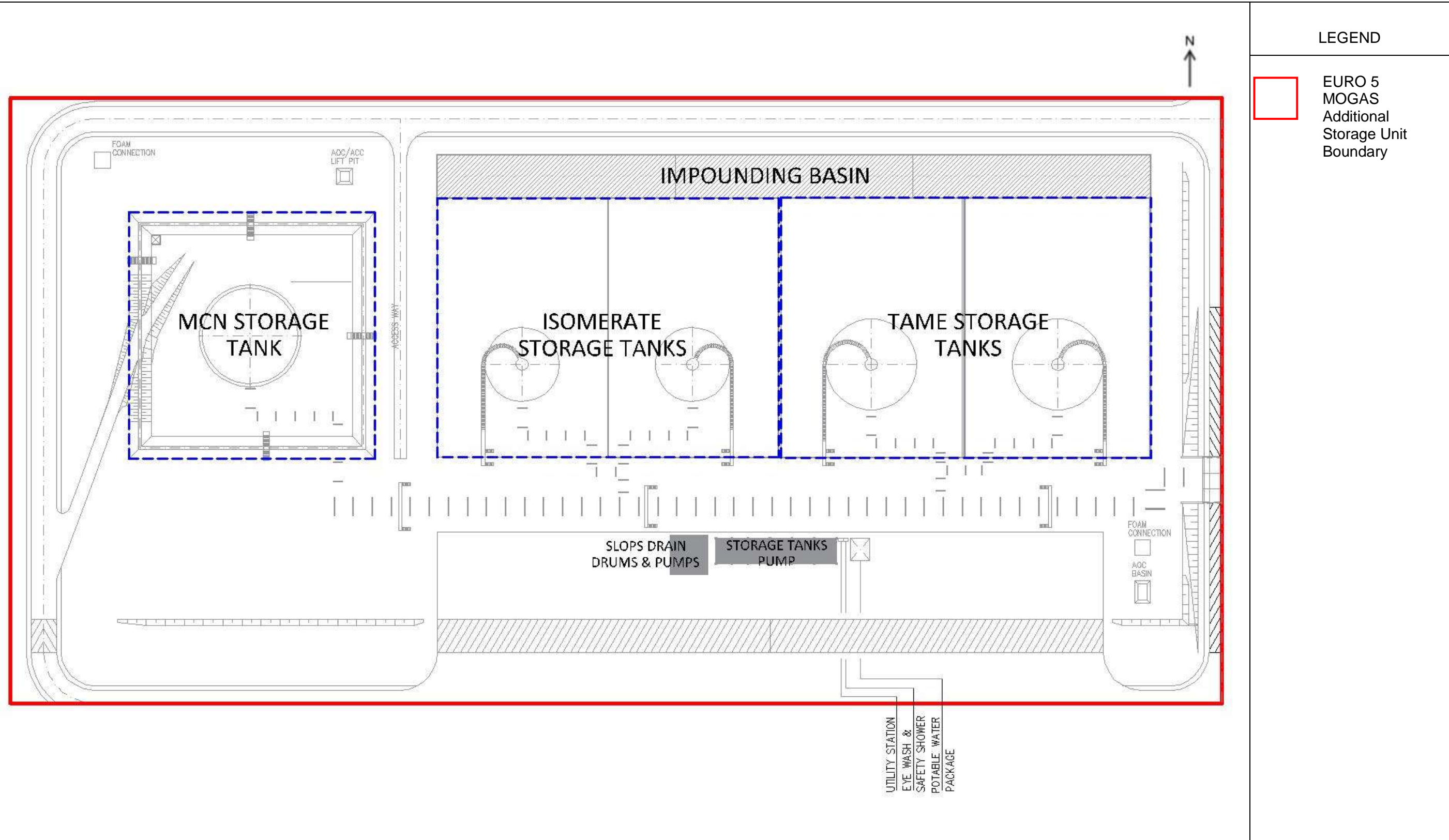
Figure 2-10: Additional Storage Tanks For EURO 5 MOGAS Unit
