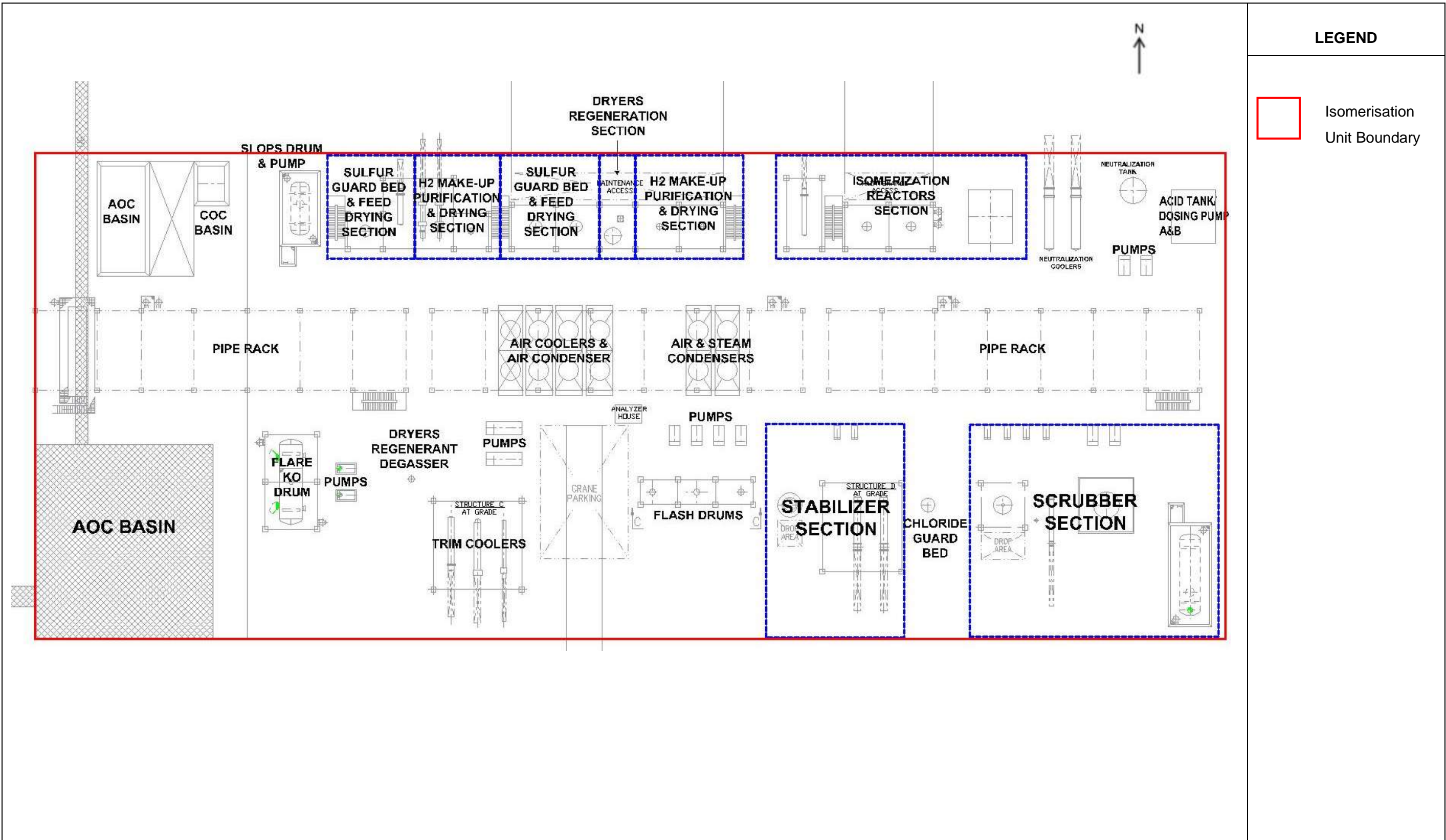
Figure 2-9: Isomerisation Unit Layout Plan
