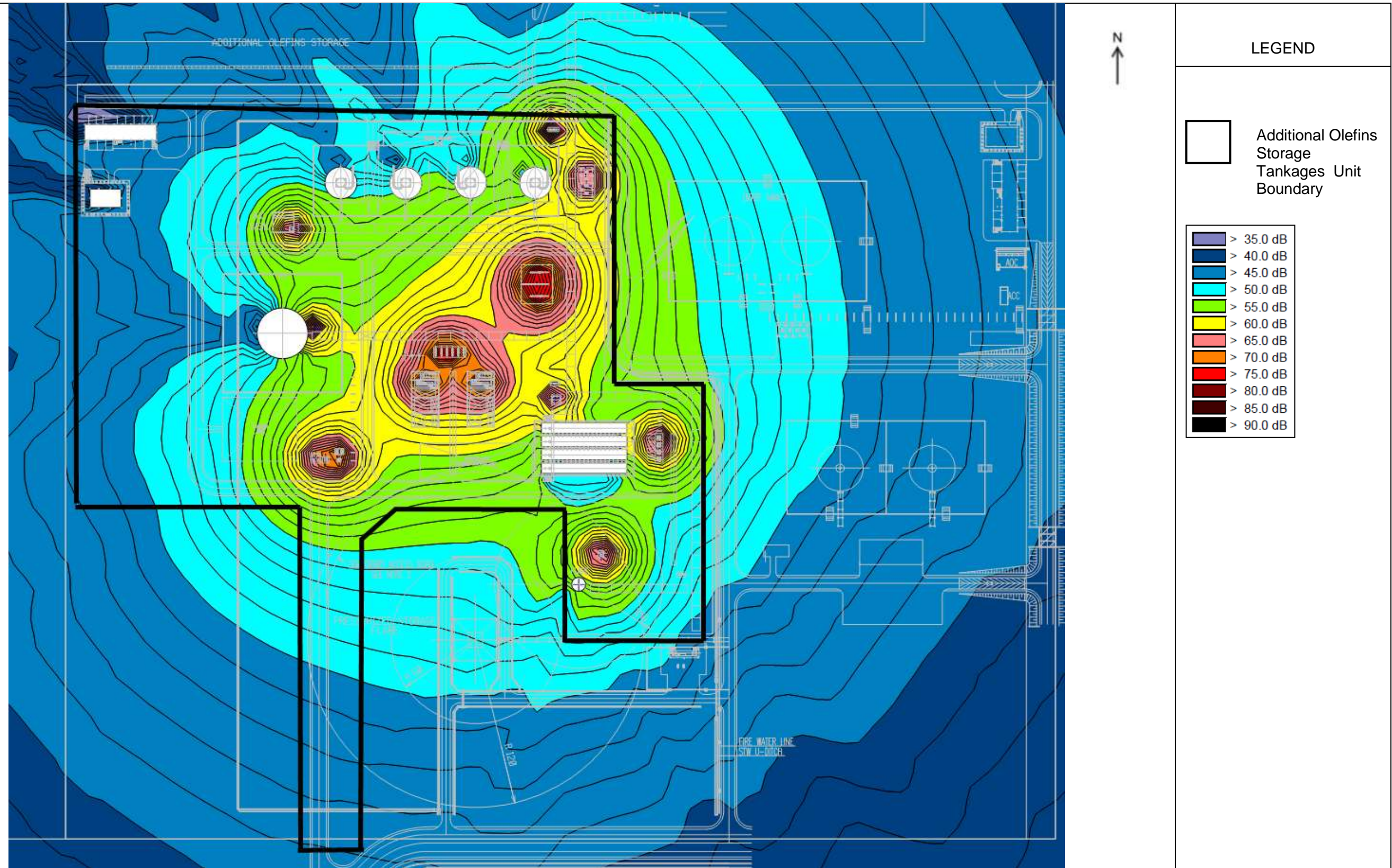
Figure 4-7: Noise Contour Generated from Additional Olefins Storage Tankages
