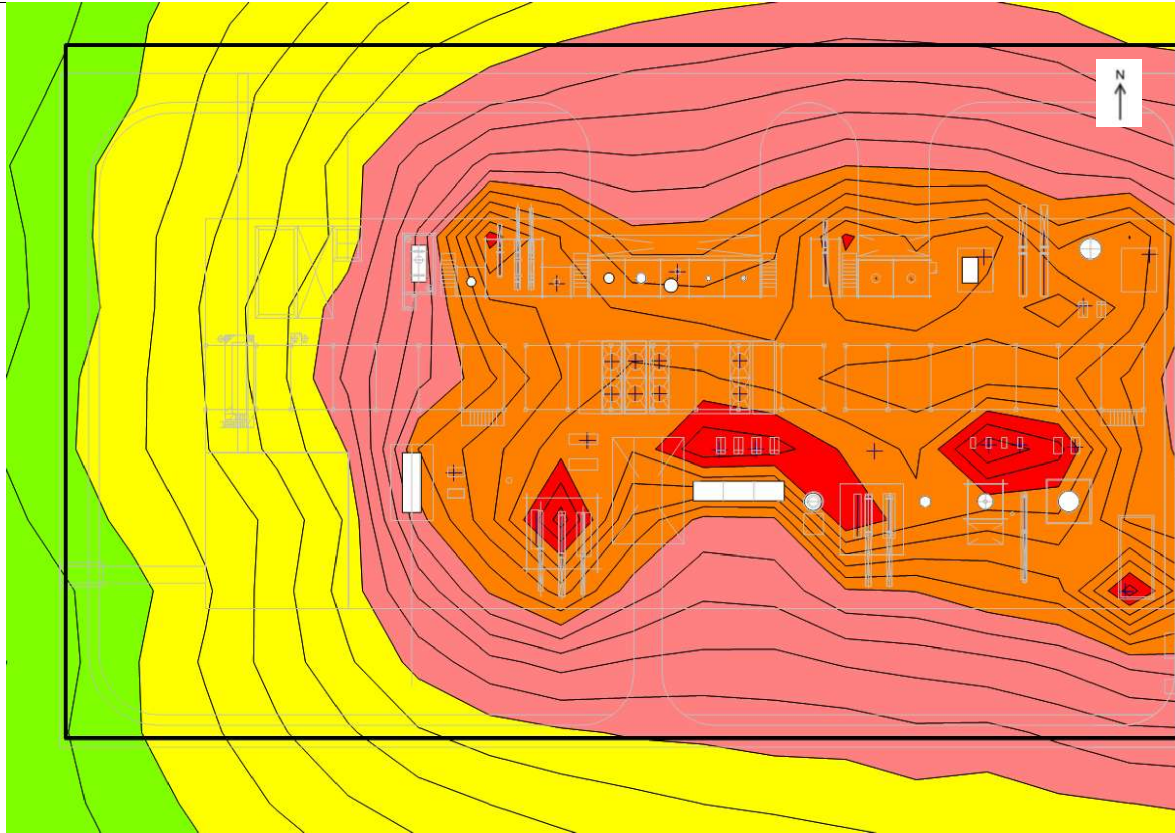
Figure 4-4: Noise Contour Generated from Isomerization Unit
