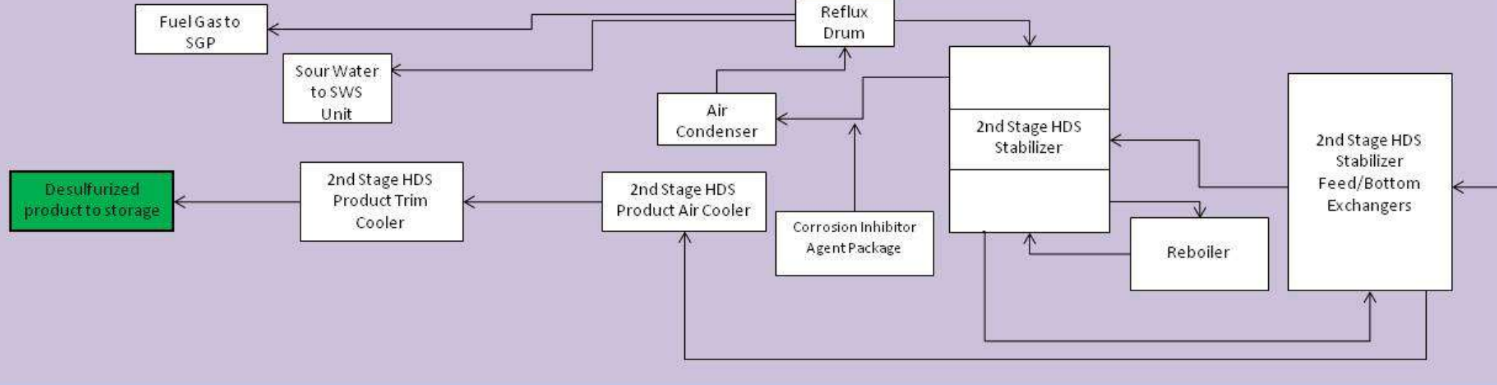
Figure 2-11: Overall Block Flow Diagram for CNHT2 Unit
