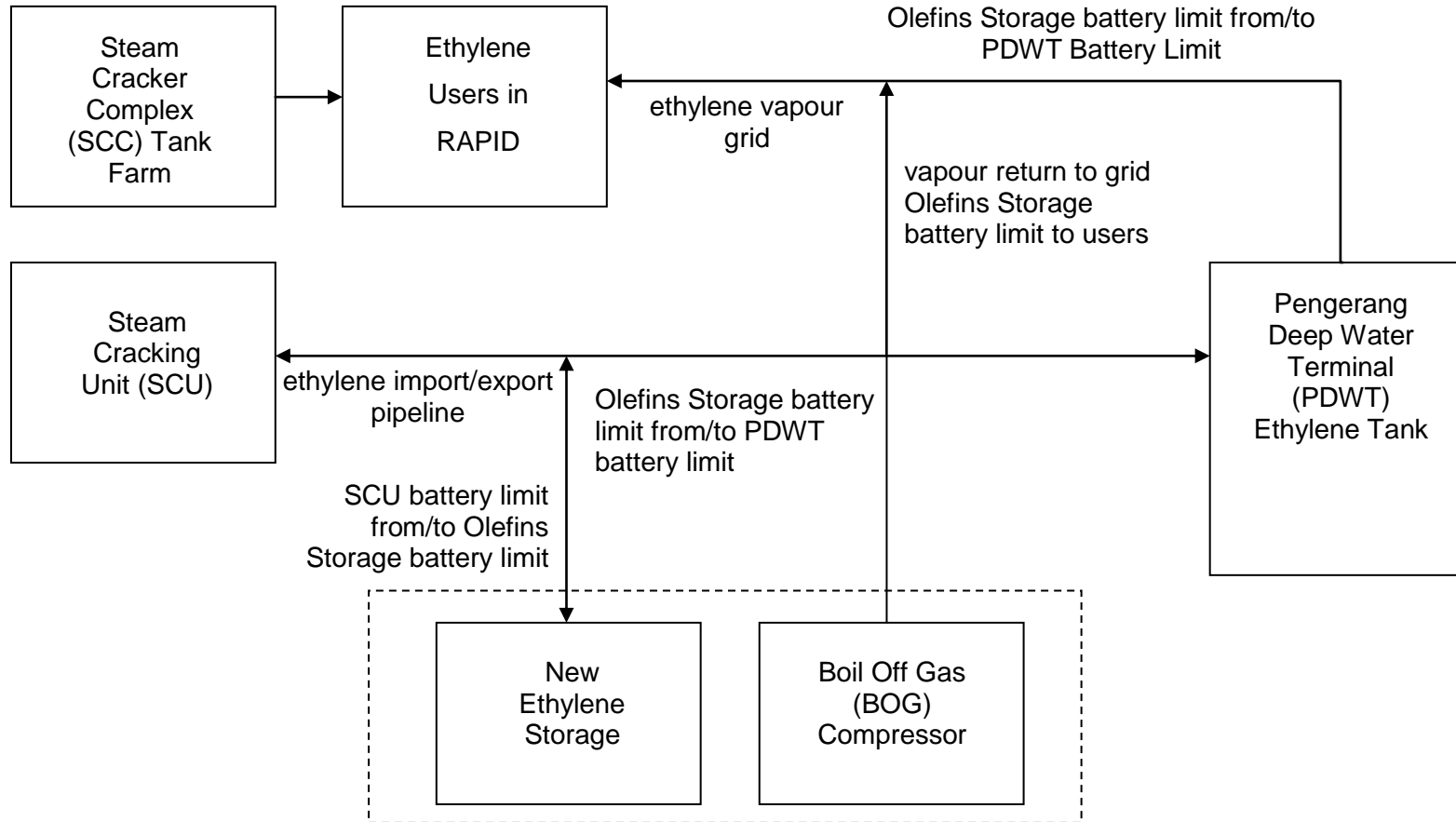
Figure 2-17: Block Flow Diagram for New Ethylene Storage
