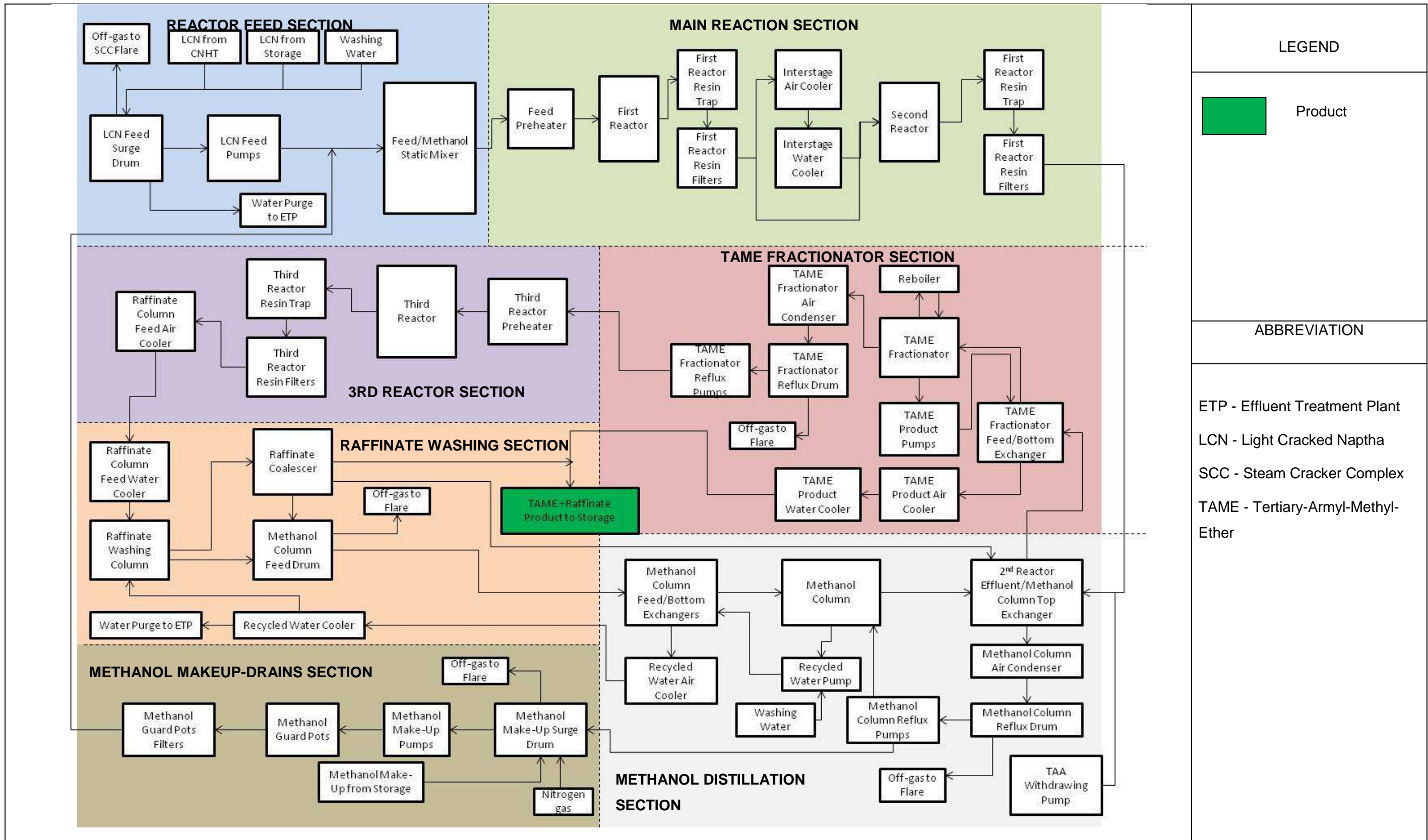
Figure 2-13: Overall Block Flow Diagram for Etherification (TAME) Unit
