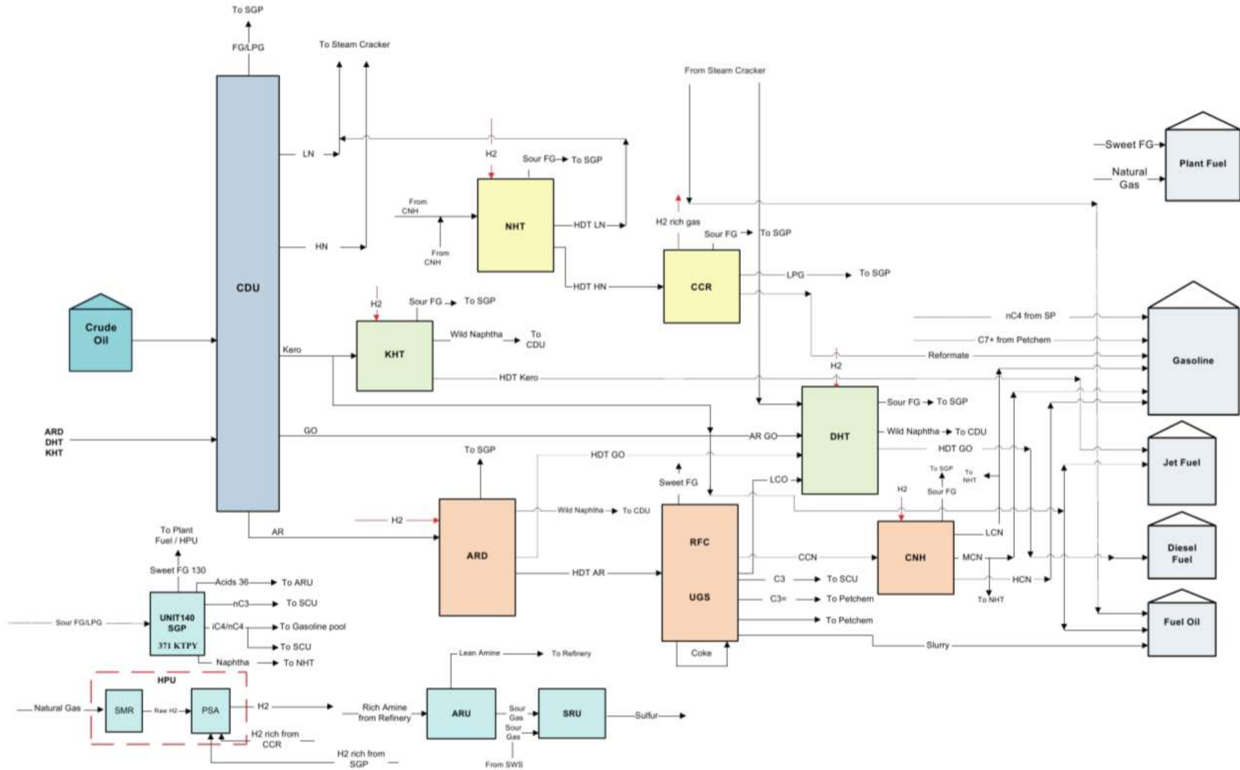
Figure 2-5: Overall Block Flow Diagram for RAPID Refinery Complex as in RAPID DEIA, 2012
