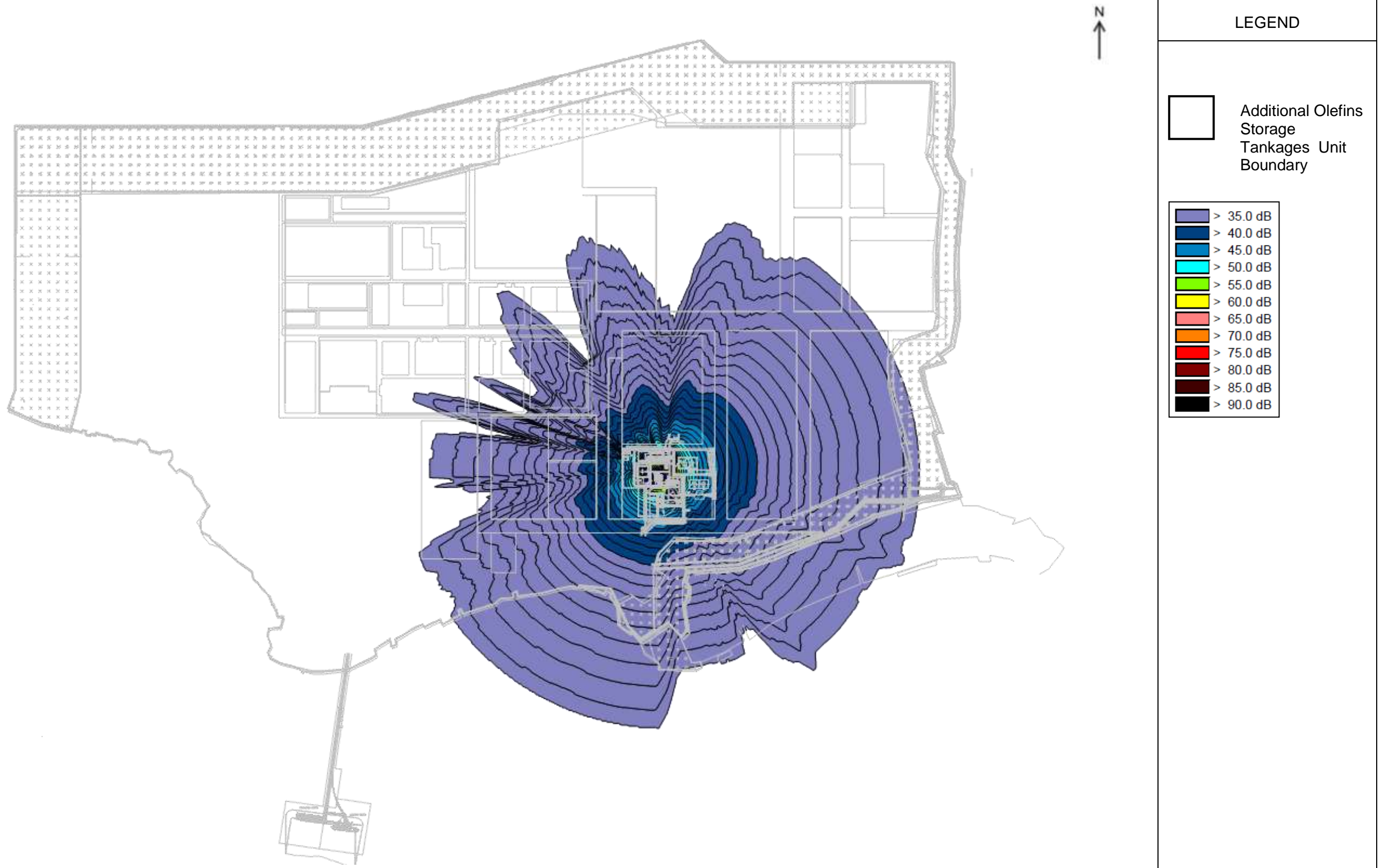
Figure 4-8: Noise Contour Generated from Olefins Storage Tankages
