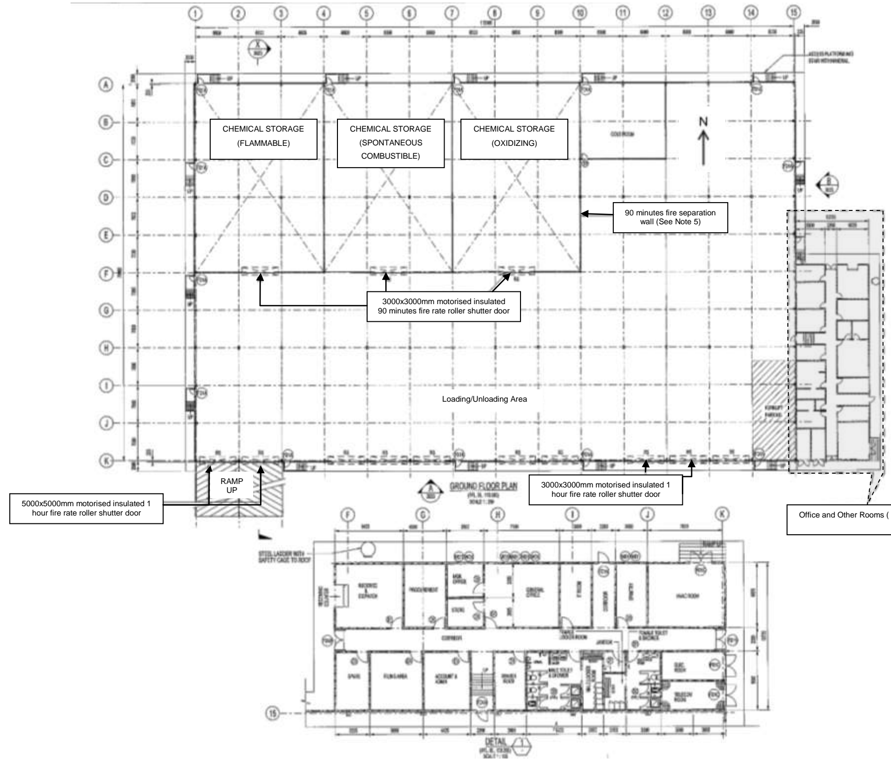
Figure 4-15 Proposed Layout of the Common Chemical Storage Warehouse
