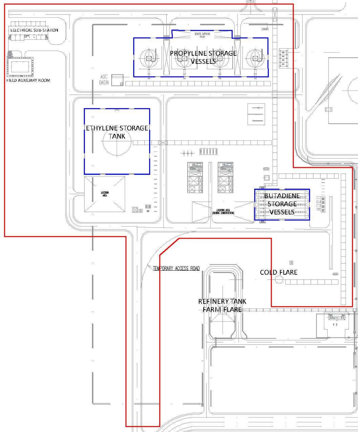
Figure 2-15: Additional Olefins Storage Layout Plan
