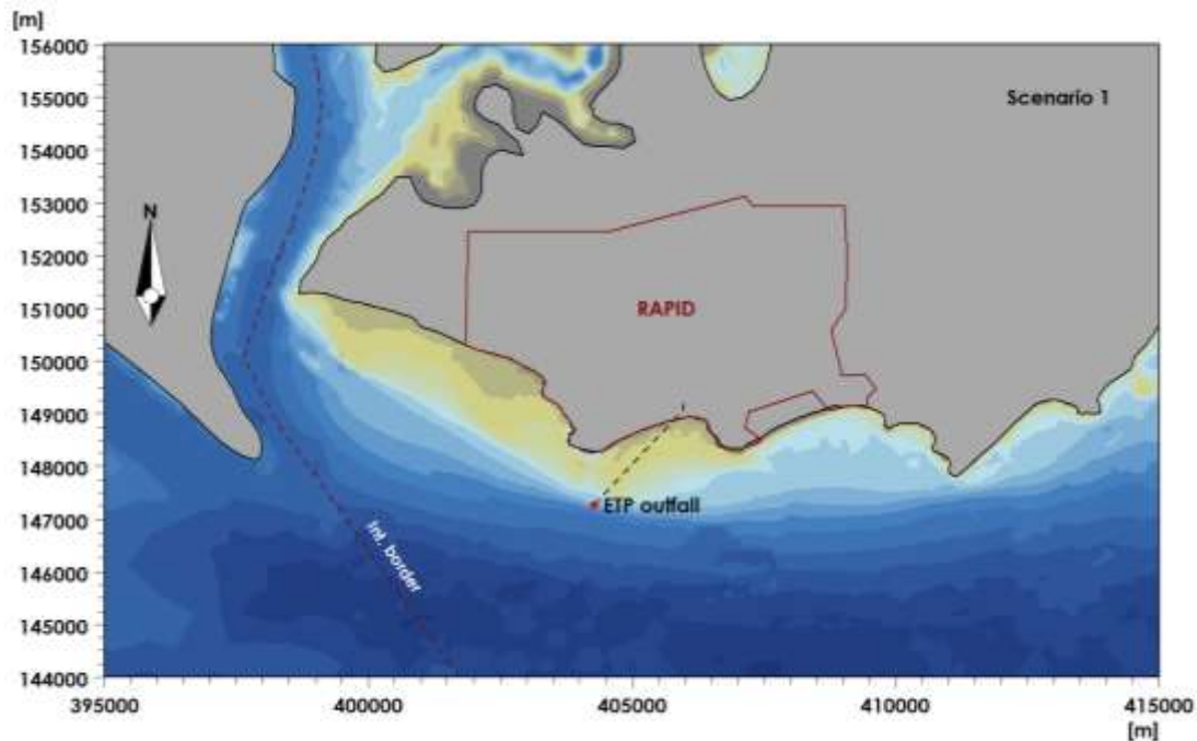
Figure 3-3: Modelled layout.
