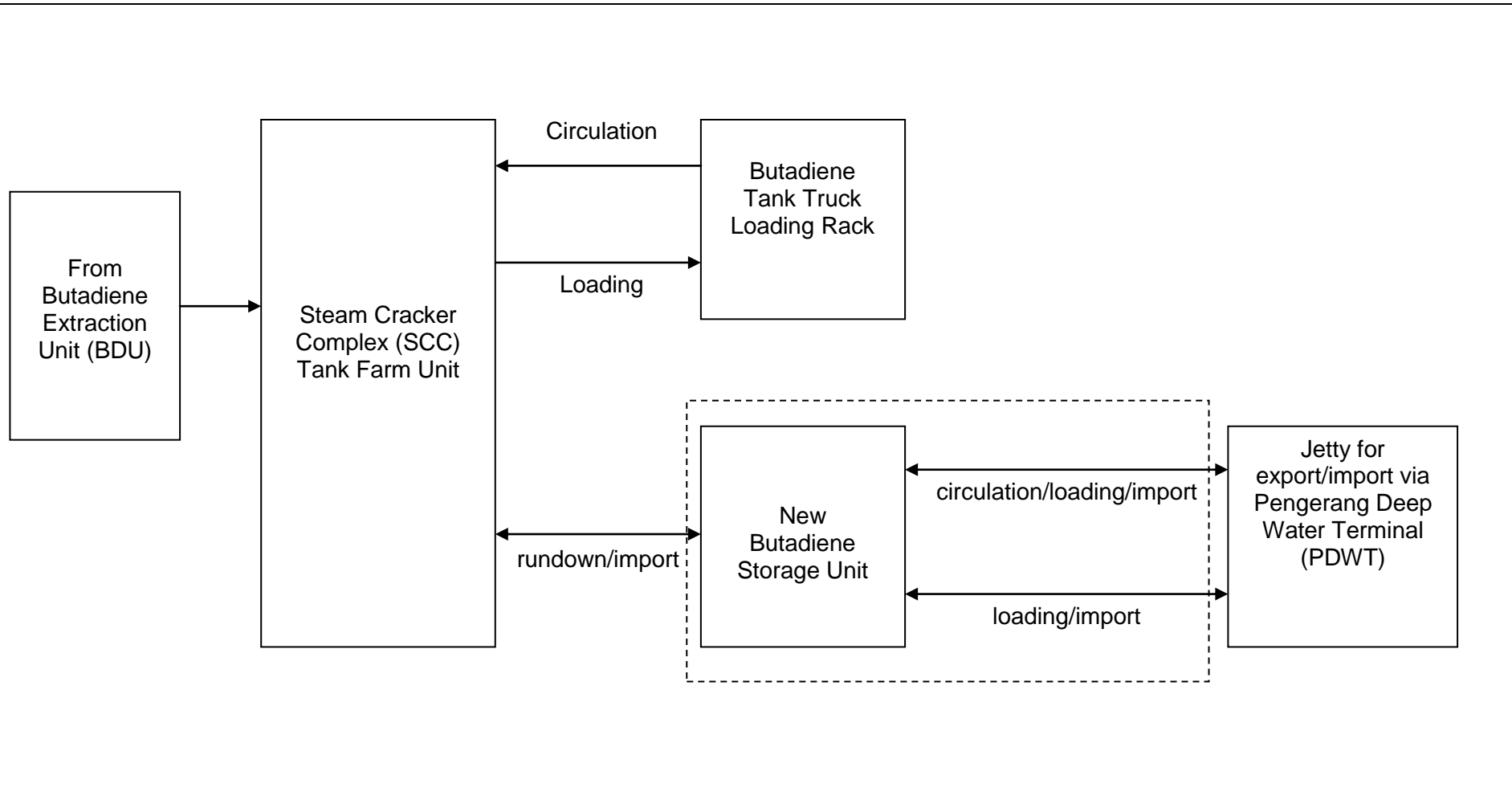
Figure 2-16: Block Flow Diagram for New Butadiene Storage Unit
