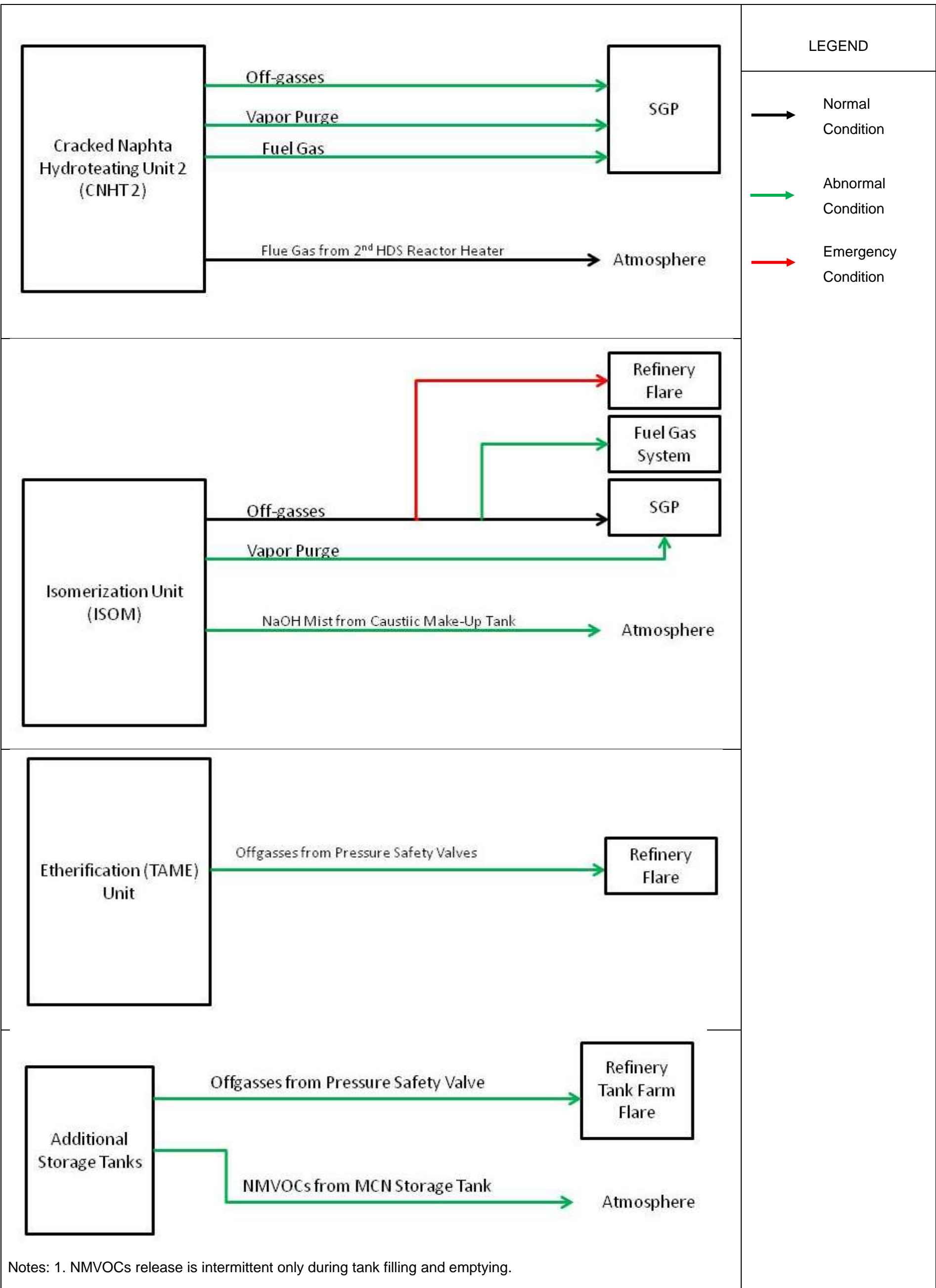
Figure 2-14: Air Emission Schematic Diagram for EURO 5 MOGAS New Units
