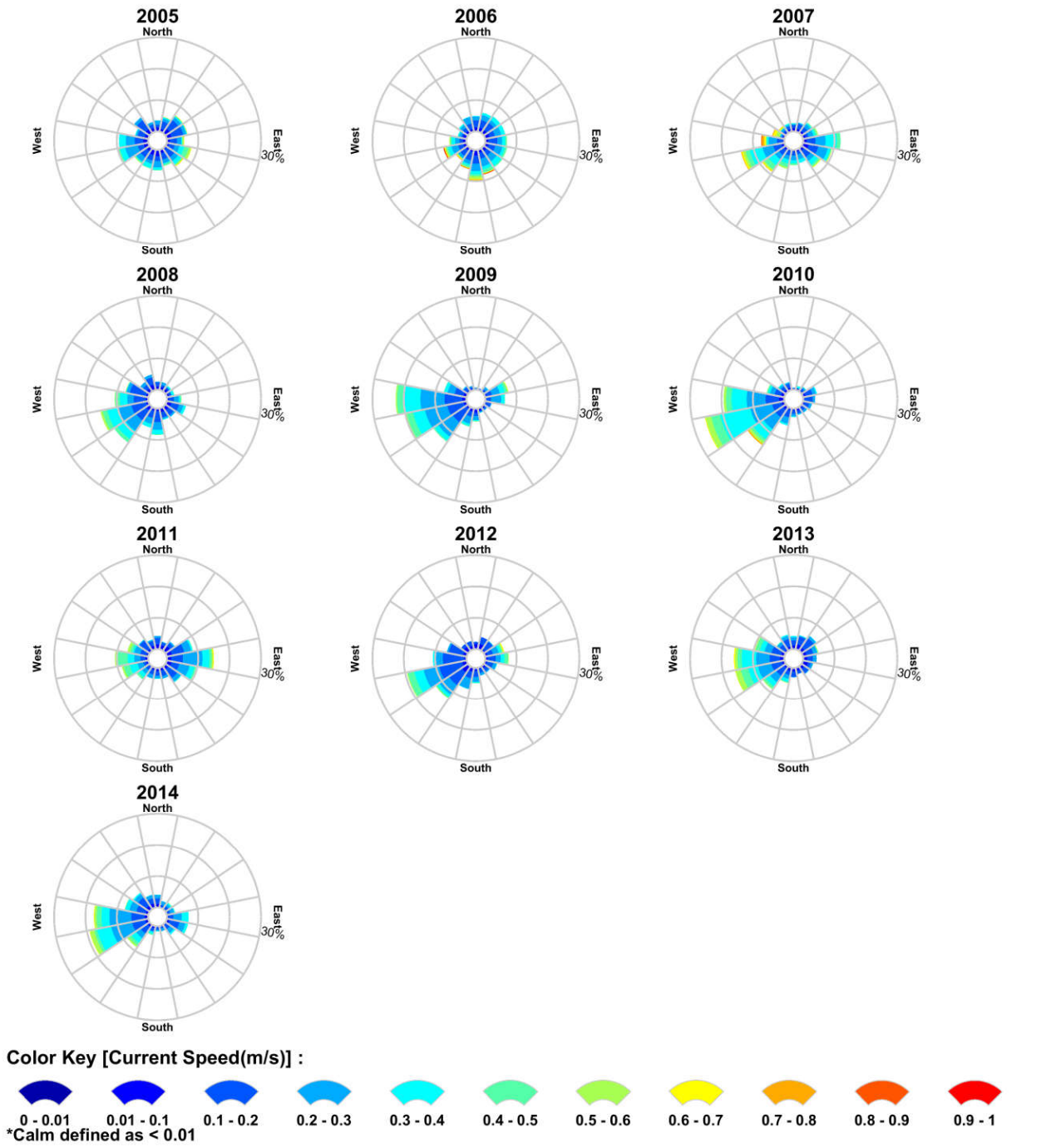
Figure 3 Annual surface ocean current rose plots within the Barossa offshore development area. Derived from analysis of HYCOM ocean data for the years 2005–2014. The colour key shows the current speed (m/s), the compass shows the direction and the length of the wedge gives the percentage of the record for a particular speed and direction combination.
