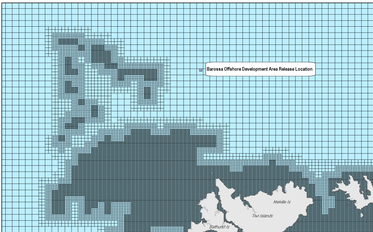
Figure 5 Zoomed in map showing the tidal model grid), illustrating the resolution sub-gridding in complex areas (e.g. islands, banks, shoals or reefs)
