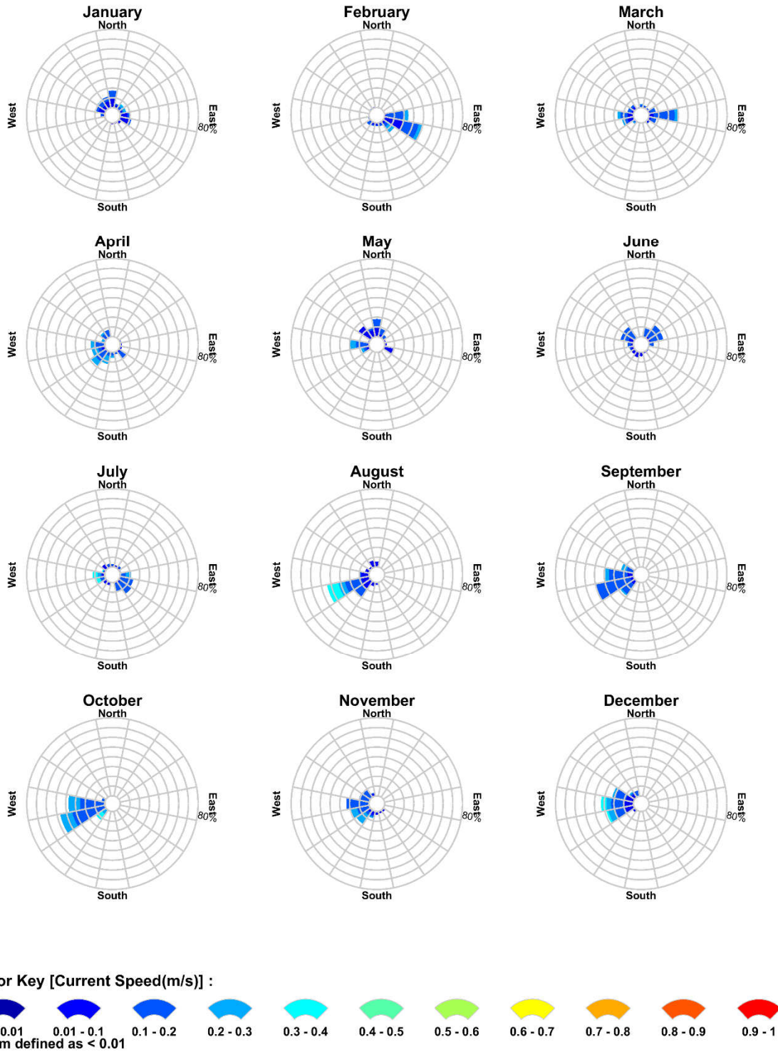
Figure 11 Monthly surface current rose plots adjacent to the model release location. Derived from analysis of HYCOM ocean data and tidal data for 2014 (El Niño year). The colour key shows the current speed (m/s), the compass shows the direction and the length of the wedge gives the percentage of the record for a particular speed and direction combination.
