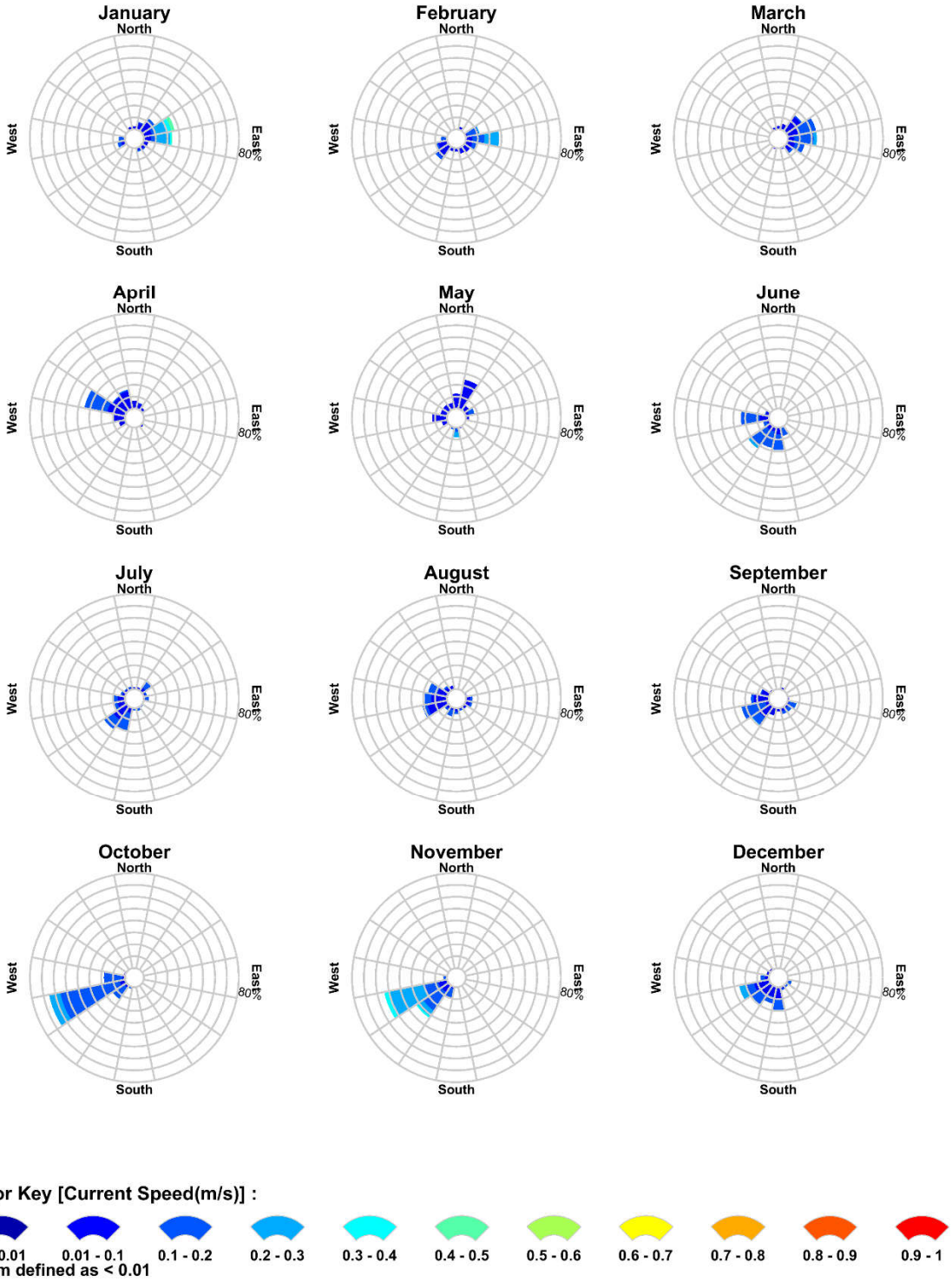
Figure 10 Monthly surface current rose plots adjacent to the model release location. Derived from analysis of HYCOM ocean data and tidal data for 2012 (neutral year). The colour key shows the current speed (m/s), the compass shows the direction and the length of the wedge gives the percentage of the record for a particular speed and direction combination.
