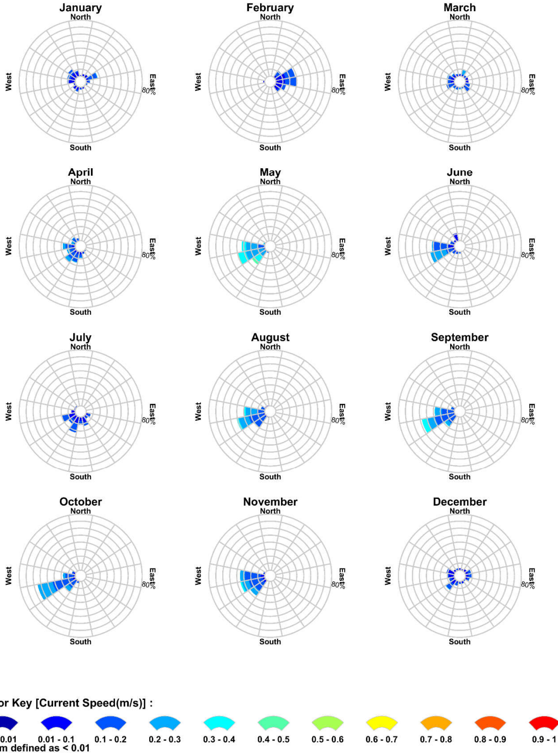
Figure 9 Monthly surface current rose plots adjacent to the model release location. Derived from analysis of HYCOM ocean data and tidal data for 2010 (La Niña year). The colour key shows the current speed (m/s), the compass shows the direction and the length of the wedge gives the percentage of the record for a particular speed and direction combination.
