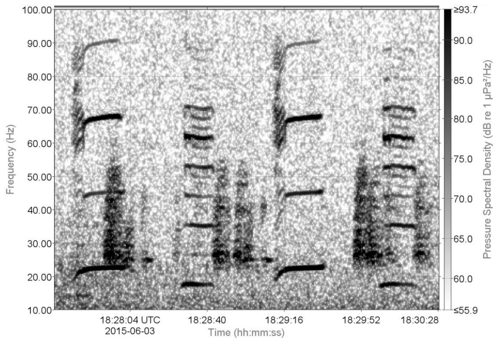
Figure 18. Spectrogram of pygmy blue whale songs showing two repetitions of each call type in sequence and Omura's whale calls in the background, recorded at Station J2 on 3 June 2015 (UTC) (0.0916 Hz frequency resolution, 2 s time window, 0.5 s time step, Hamming window).
