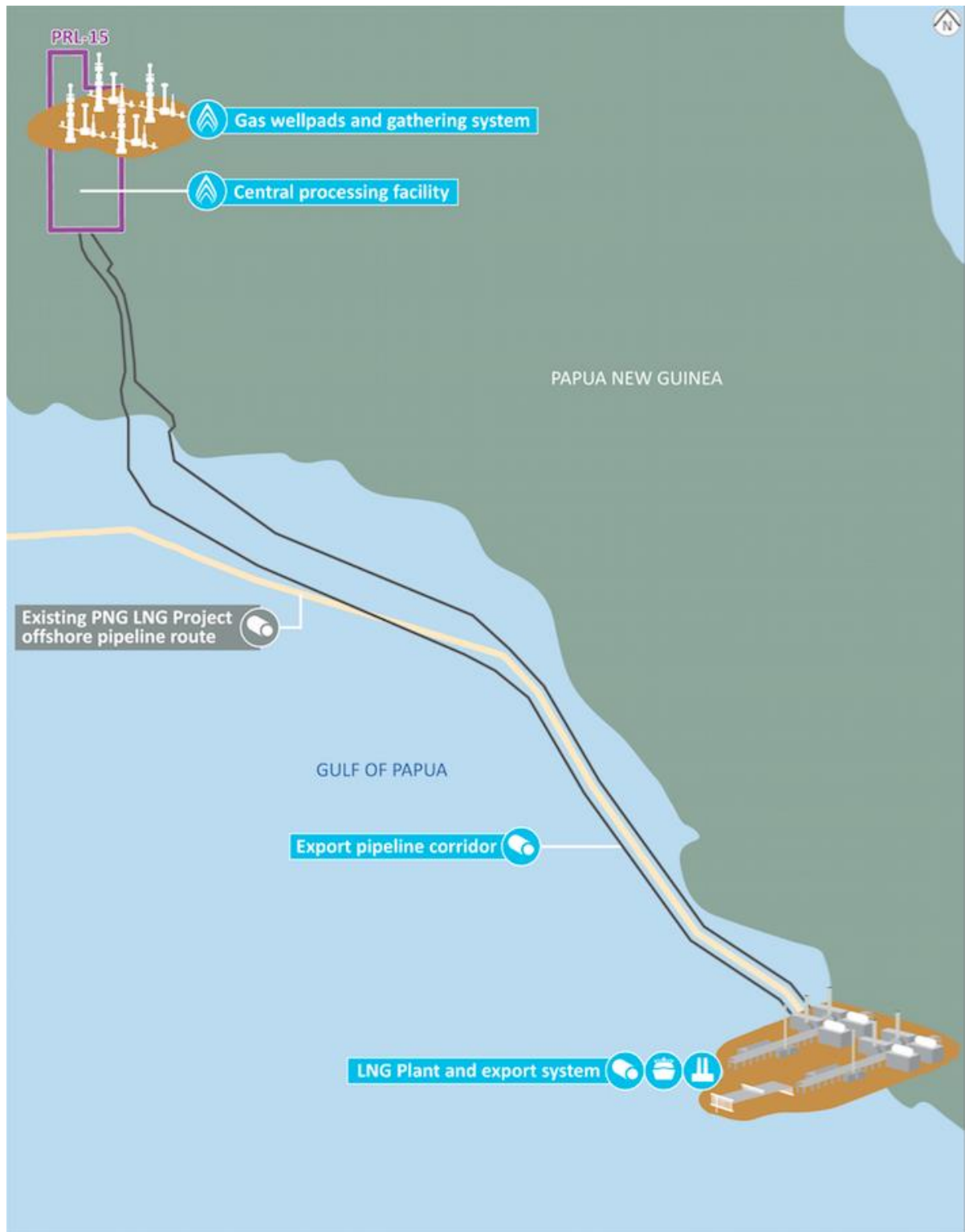
Figure 1.1 – Project Schematic
