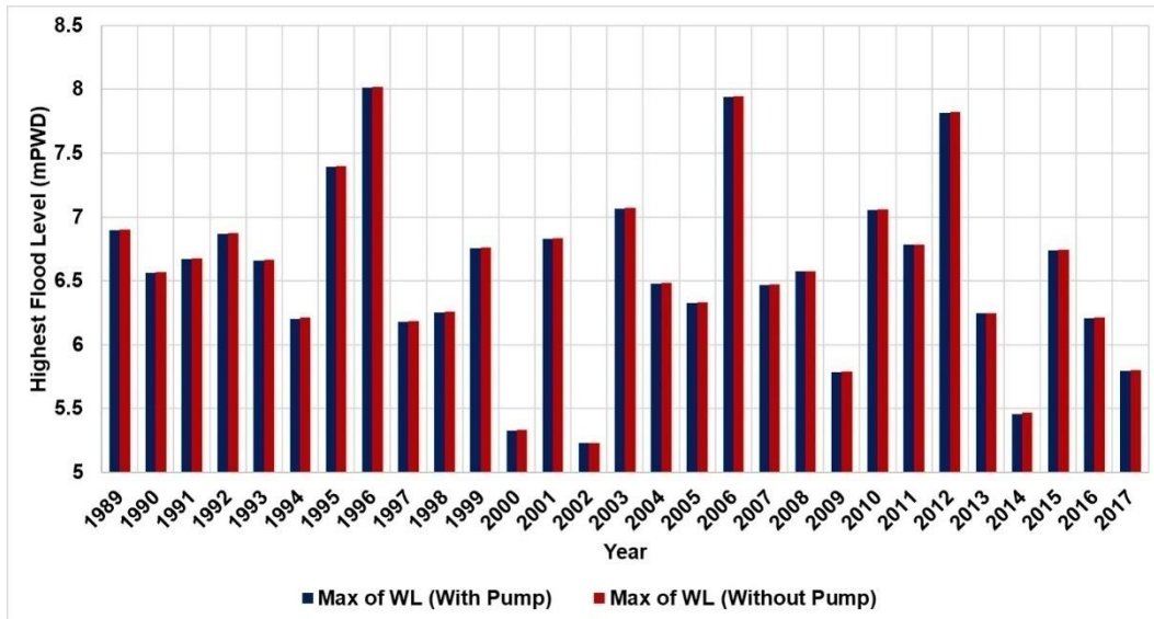
Figure 7.5: Highest Flood Level With and Without Pump
