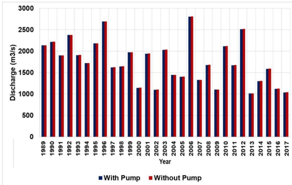
Figure 7.7: High Discharge Rate With and Without Pump
