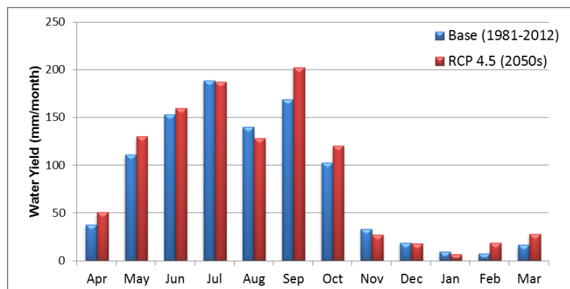
Figure 7.2: Climate change impact on monthly water yield for climate scenario RCP 4.5 by 2050s
